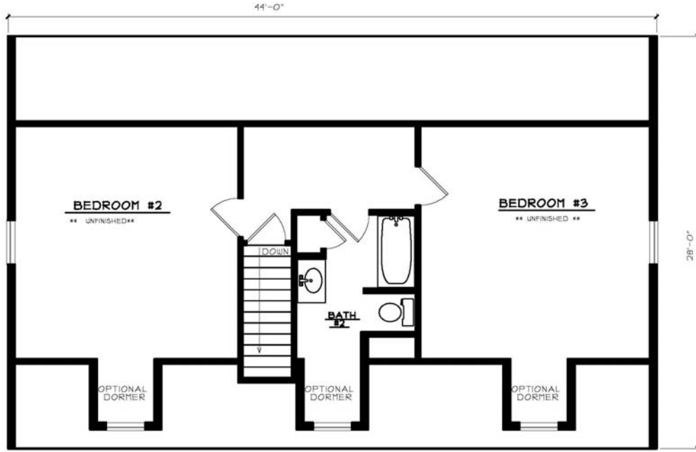
SUGGESTED SECOND FLOOR PLAN
