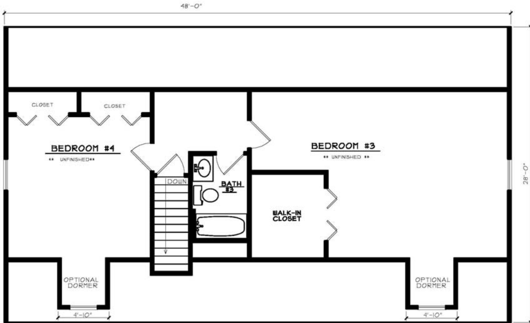
SUGGESTED SECOND FLOOR PLAN 160 SQ. FT. (UNFINISHED)
