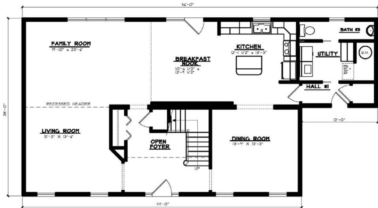
FIRST FLOOR PLAN 1400 SQ. FT.
