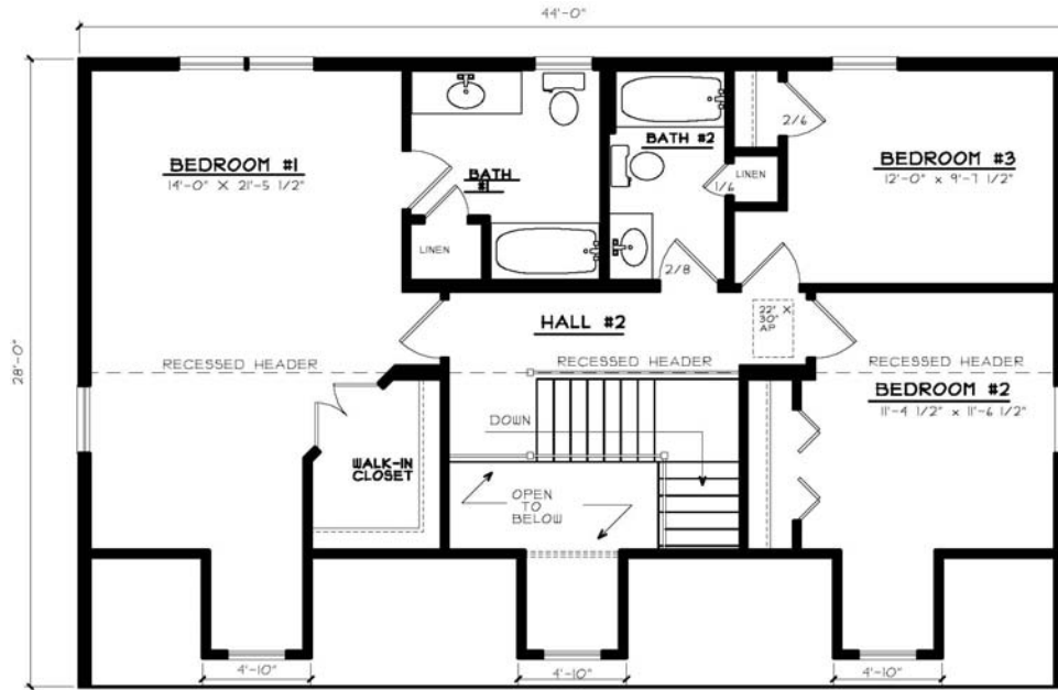
SECOND FLOOR PLAN 932 SQ. FT. (FINISHED)
