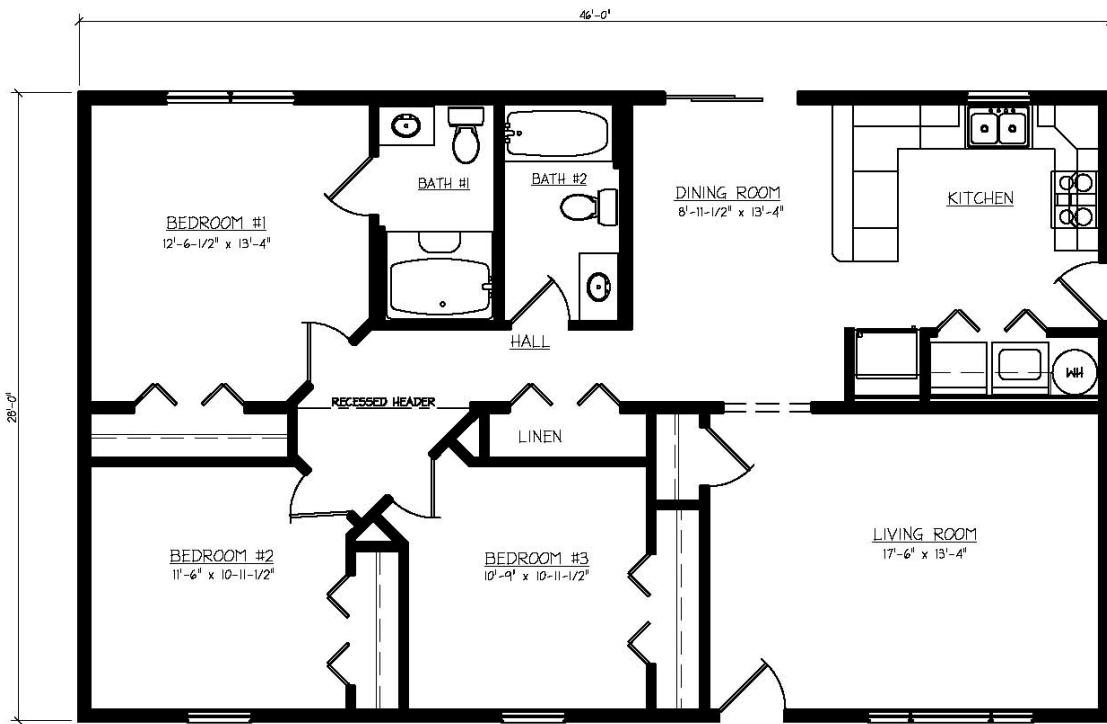
FLOOR PLAN 1288 SQ. FT. - LIVING
