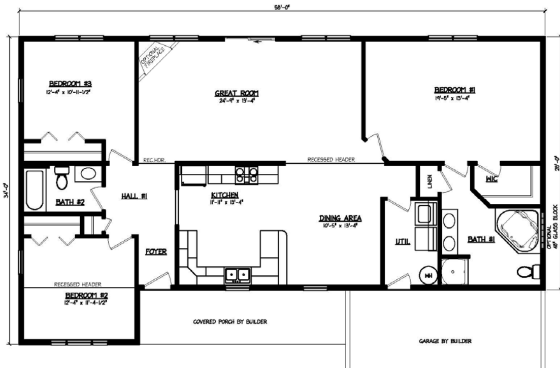
FLOOR PLAN 1703 SQ. FT. - LIVING
