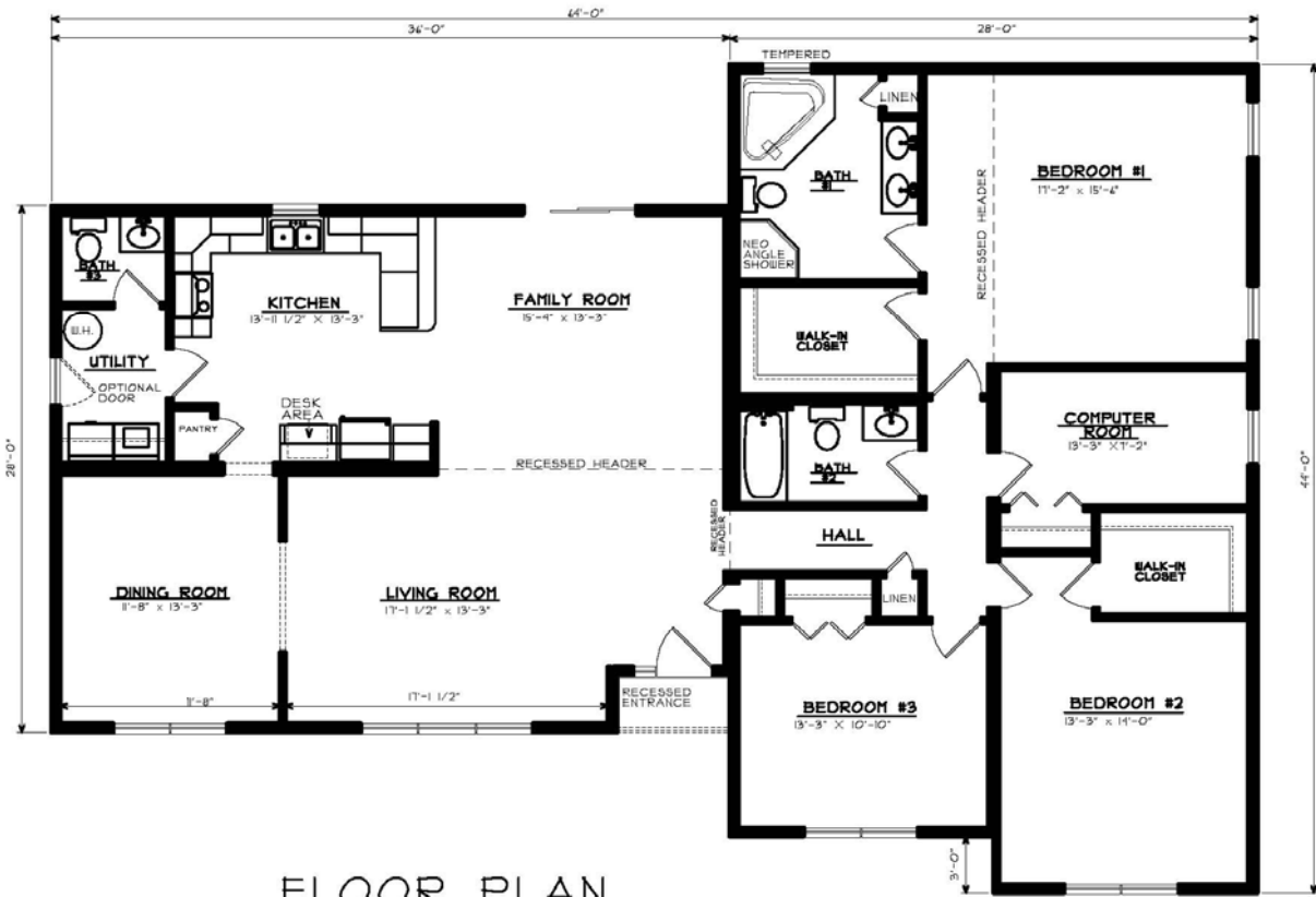
FLOOR PLAN 2198 SQ. FT. - LIVING
