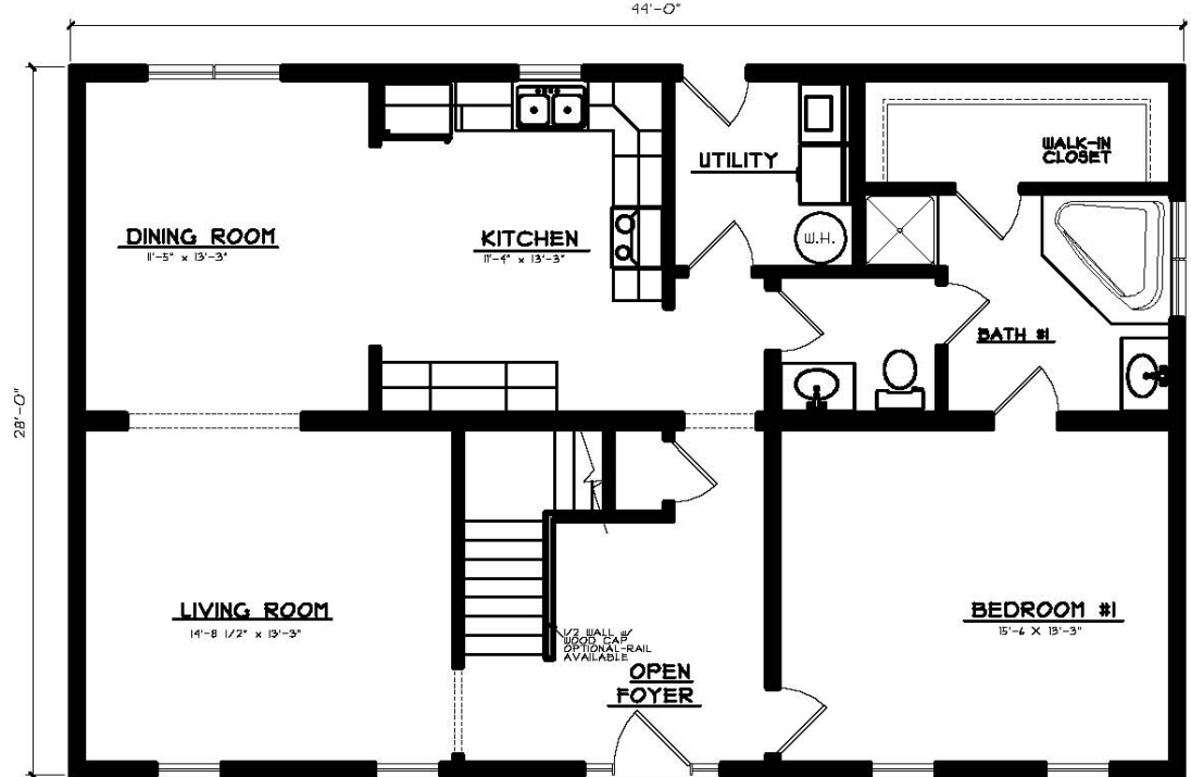
FIRST FLOOR PLAN 1232 SQ. FT.
