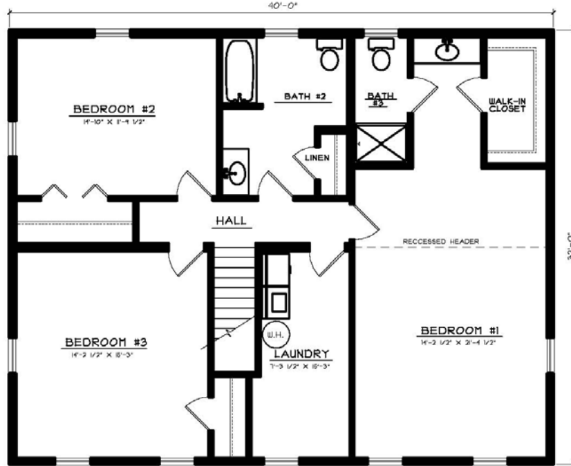
SECOND FLOOR PLAN 1280 SQ. FT.
