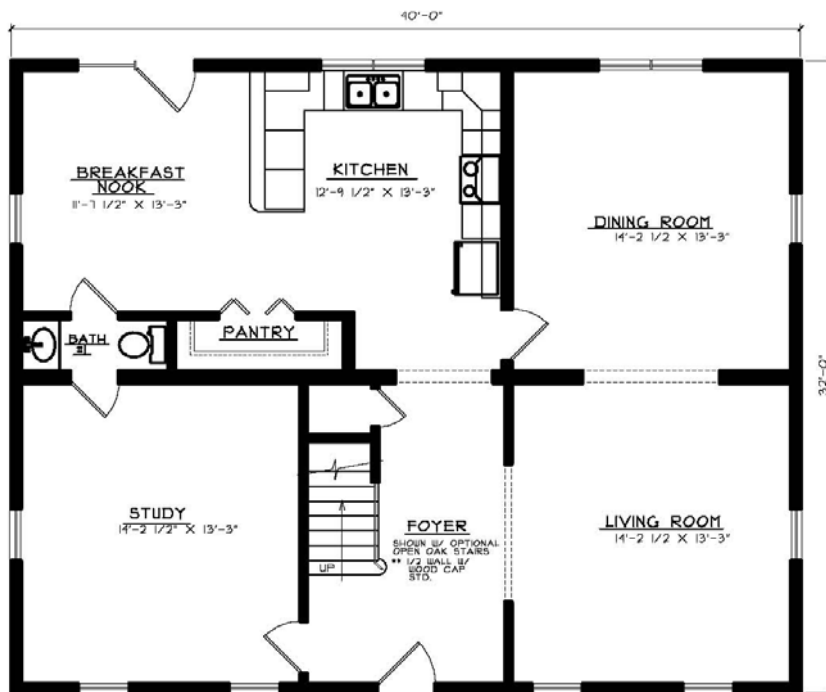
FIRST FLOOR PLAN 1280 SQ. FT.
