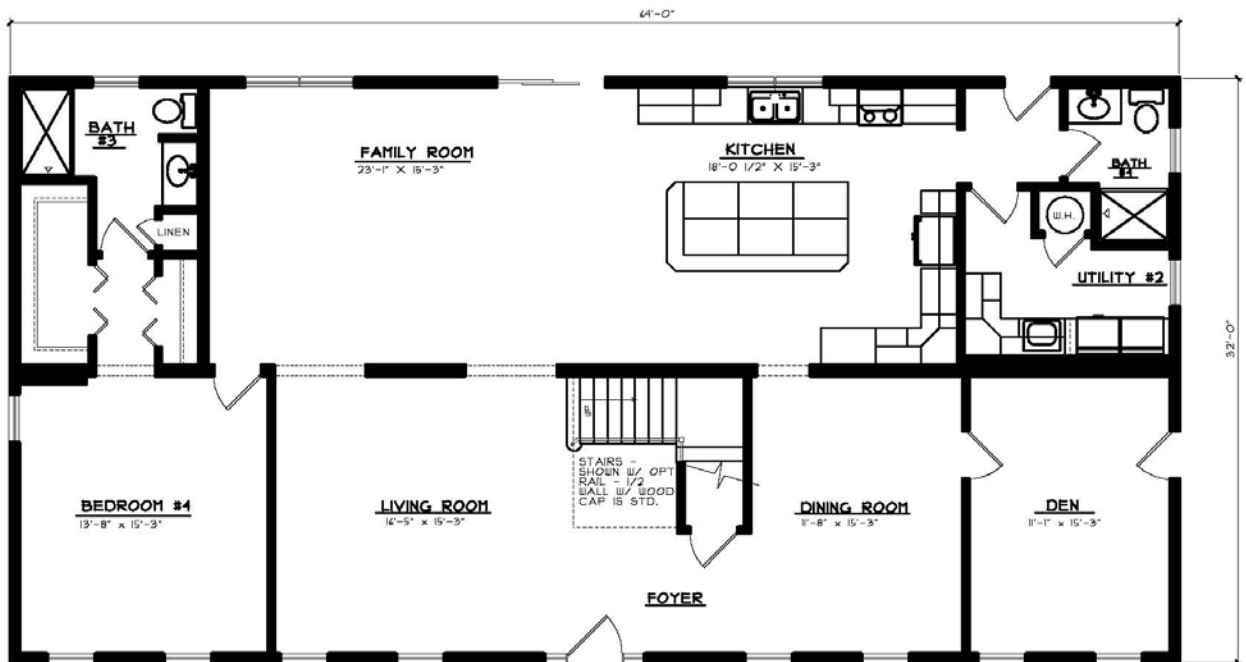
FIRST FLOOR PLAN 2048 SQ. FT.
