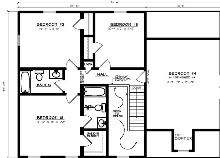
SUGGESTED SECOND FLOOR
